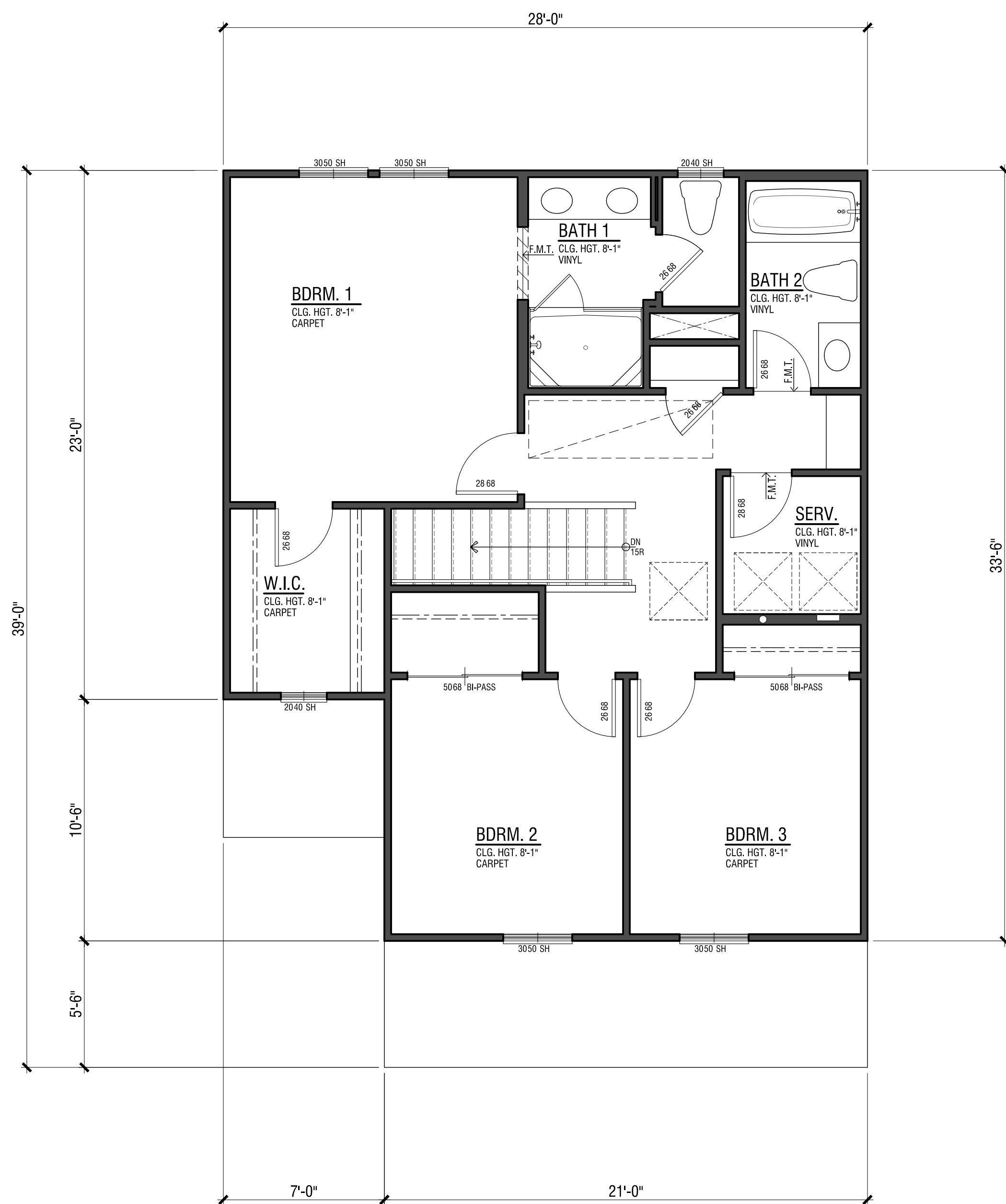
Upper Floor - 831 SF
