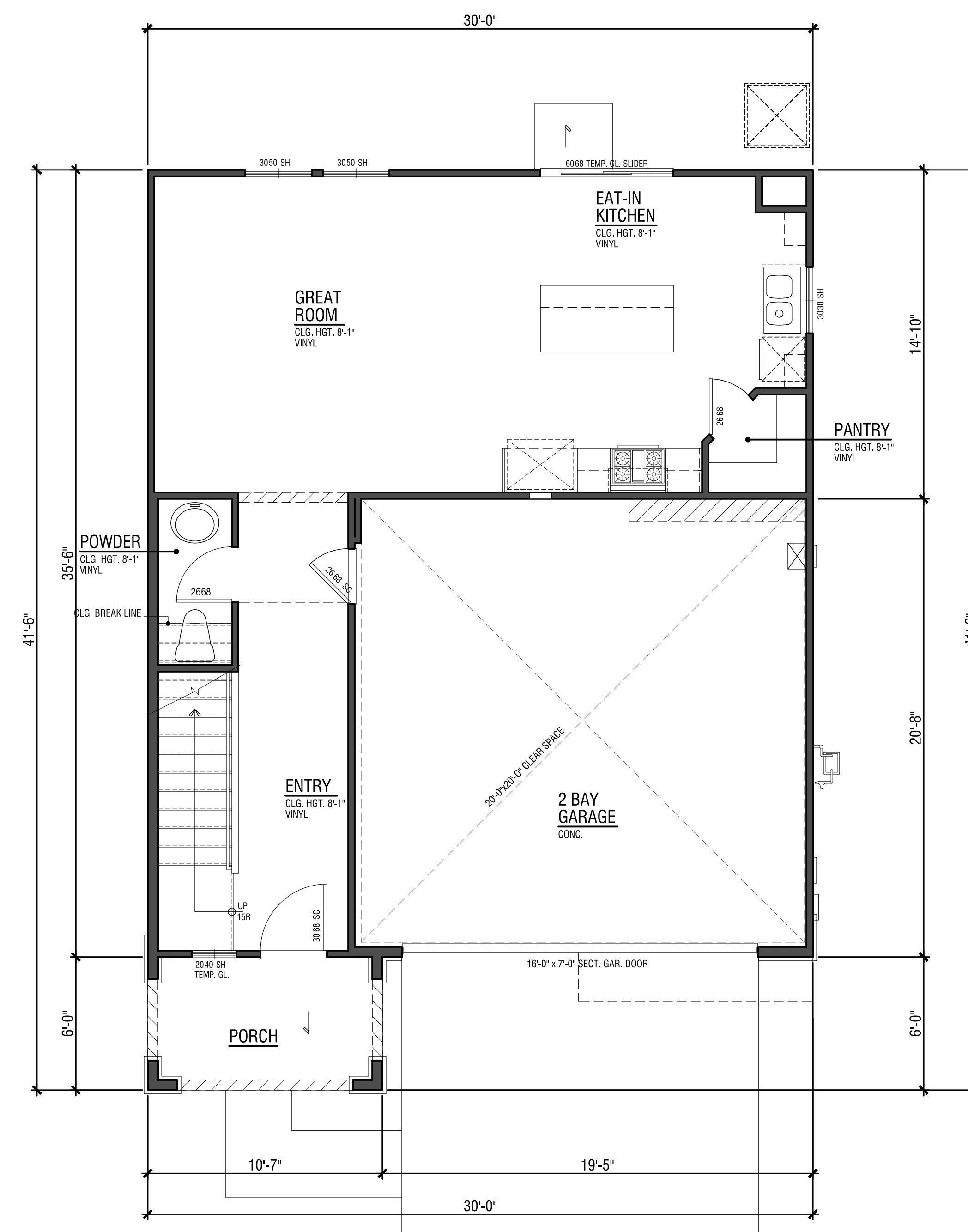
Lower Floor - 637 SF
