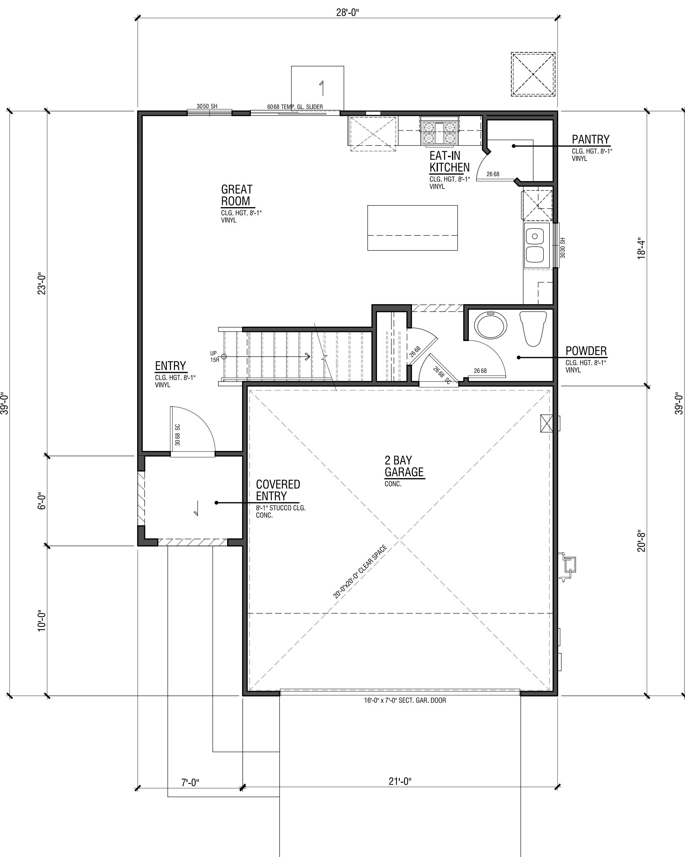
Lower Floor - 547 SF
