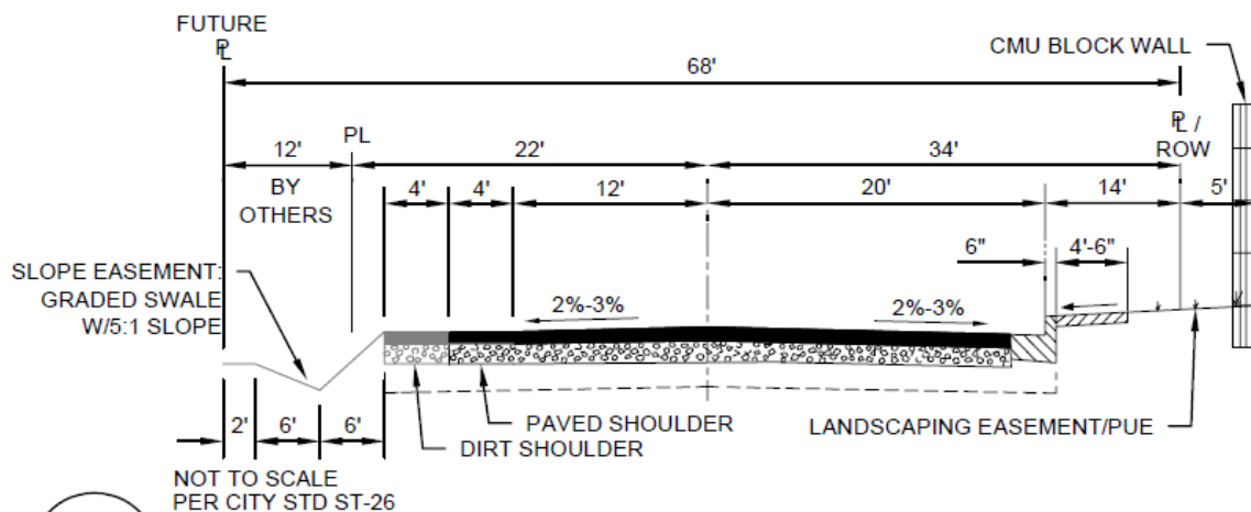
Figure 7: Street Cross-Sections
