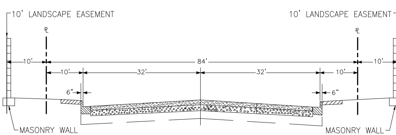
SEC. A-A MILLENNIUM WAY PER CITY STD. ST-23
