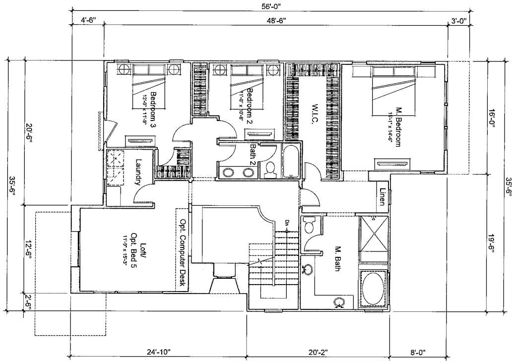
SECOND FLOOR
