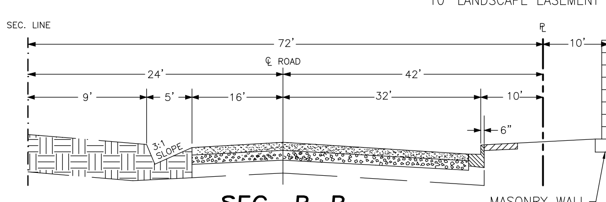
SEC. B-B 12-1/2 AVE (LOOKING NORTH) PER CITY STD. ST-23
