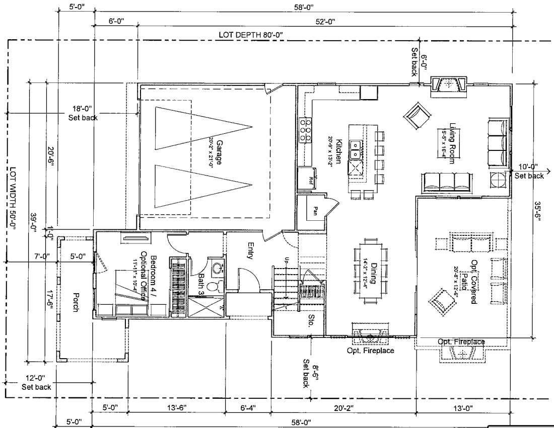
FIRST FLOOR
