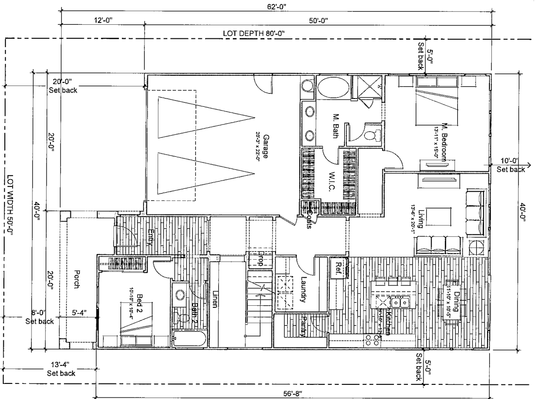
PLAN IX - FIRST FLOOR PLAN
