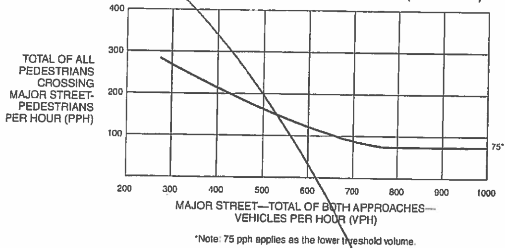
Figure 4C-6. Warrant 4, Pedestrian Four-Hour Volume (70% Factor)
