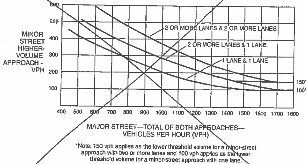
Figure 4C-3. Warrant 3, Peak Hour
